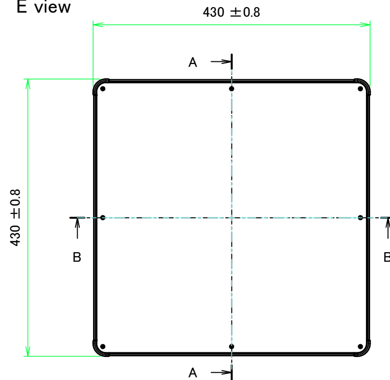
E view
